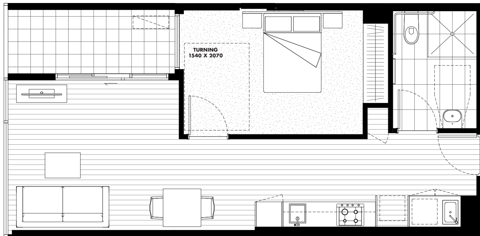
ADAPTABLE APARTMENT
